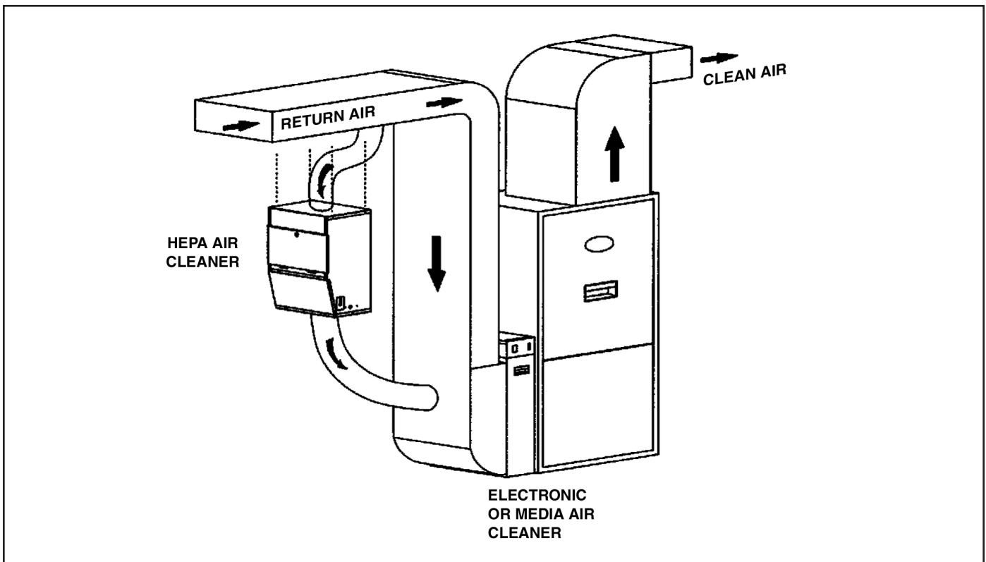
Figure 2. Collar Mount Installation
