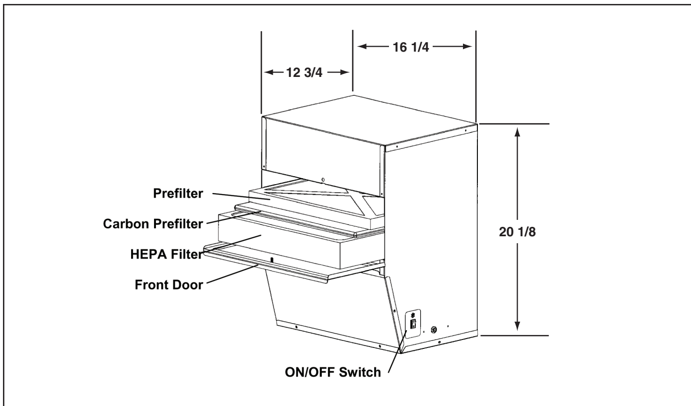
Figure 3. Whole Home Duct Mount HEPA
