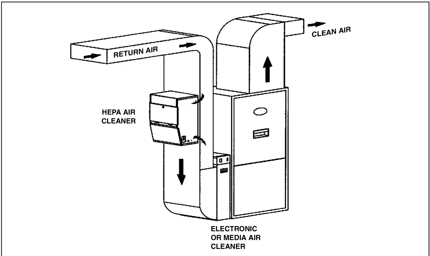
Figure 1. Duct Mount Installation
