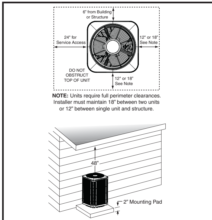
Figure 1. Clearance Requirements
