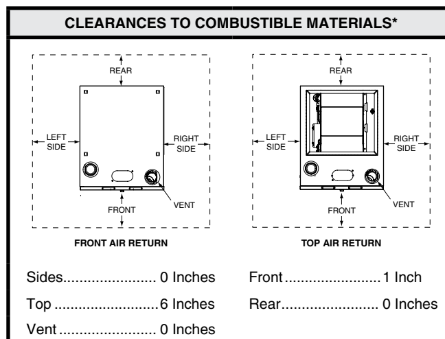
Figure 1. Minimum Clearances
