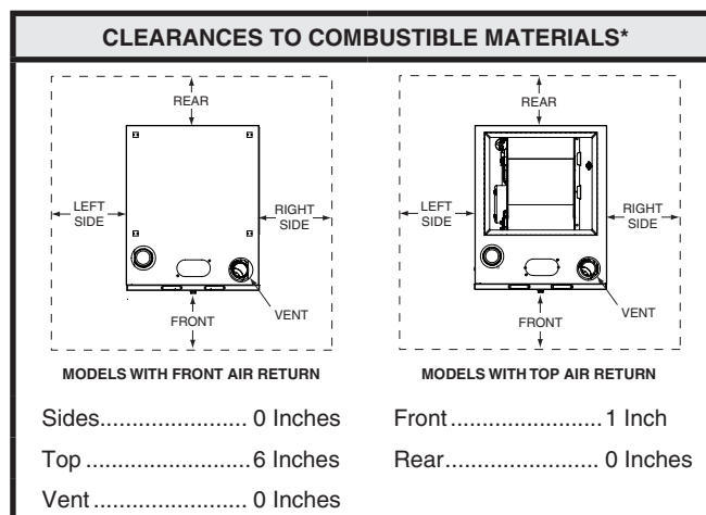
Figure 1. Minimum Clearances
