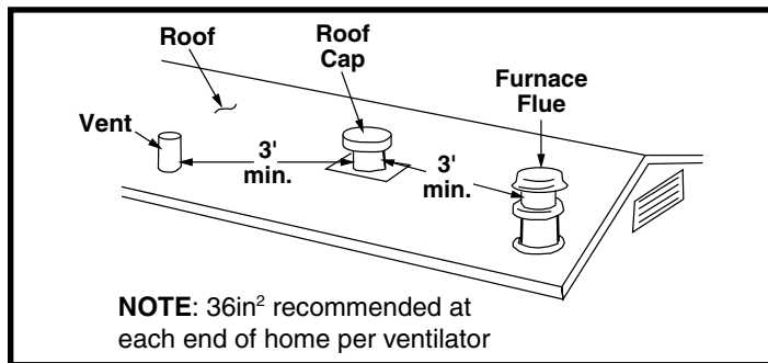
Figure 5. Roof Spacing
