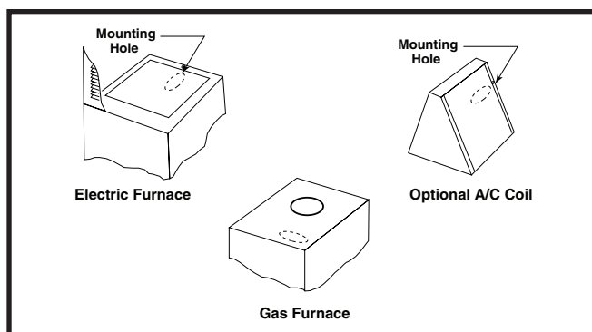
Figure 1. Plastic Inlet Fitting Location
