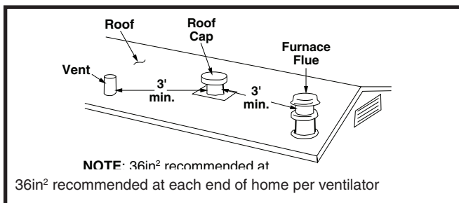
Figure 4. Roof Spacing
