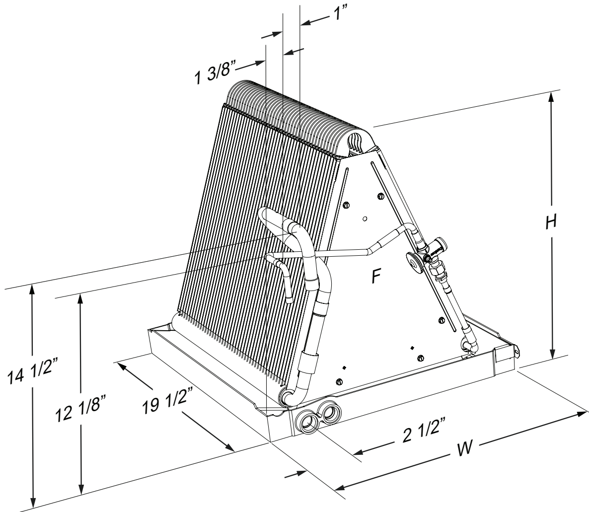
Figure 2. C84DA Coil Dimensions
