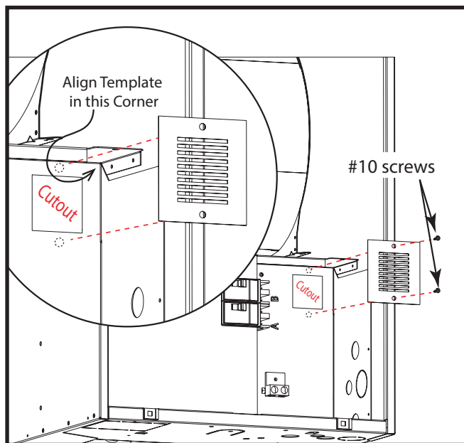
Figure 2. Control Panel Vent Plate
