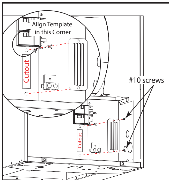
Figure 3. Control Door Vent Plate
