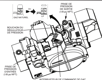
Valve de gaz Copeland
