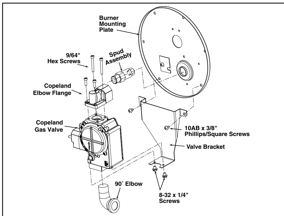
Figure 1. Burner Assembly
