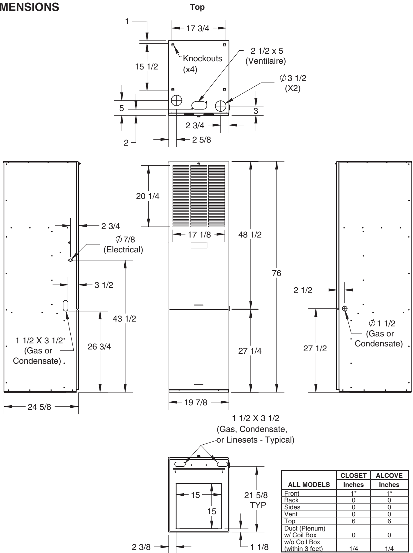
Minimum Clearances
