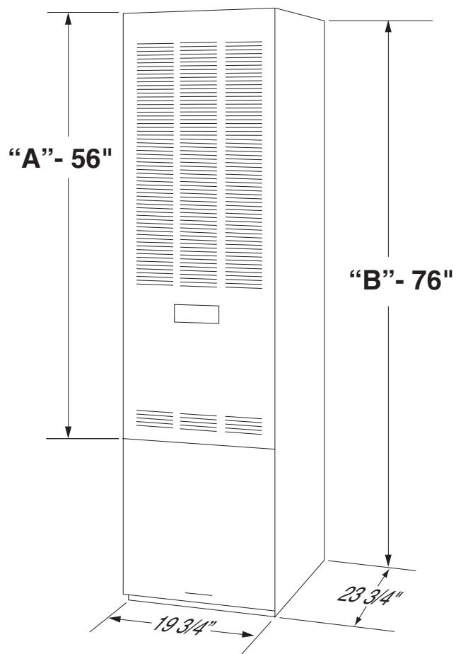
“A” Model without Coil Cabinet “B” Model with Coil Cabinet
