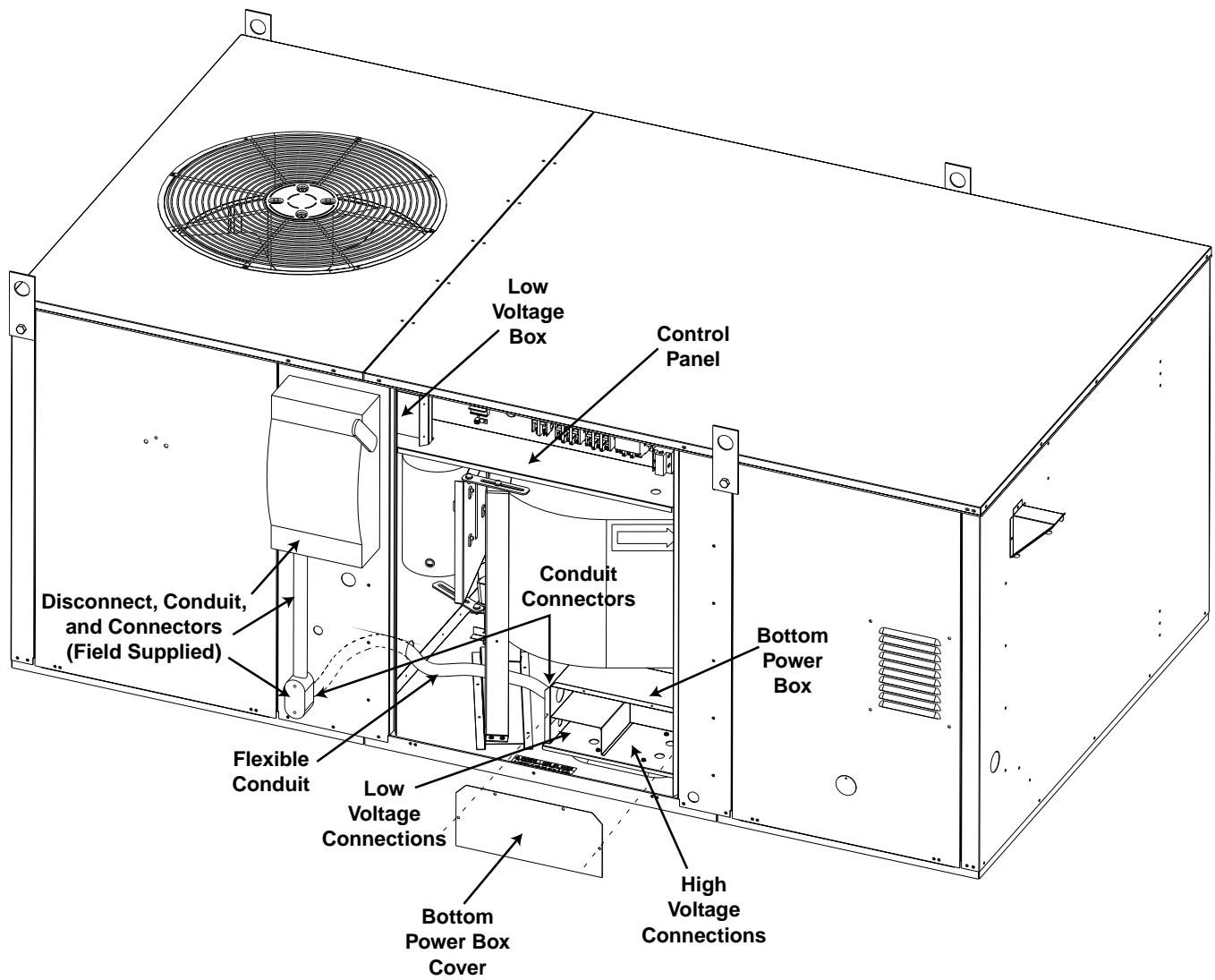
Figure 1. R4GM Bottom Power Entry Kit
