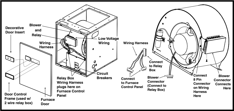
Figure 1. E1E(-) Series Electric Furnace
