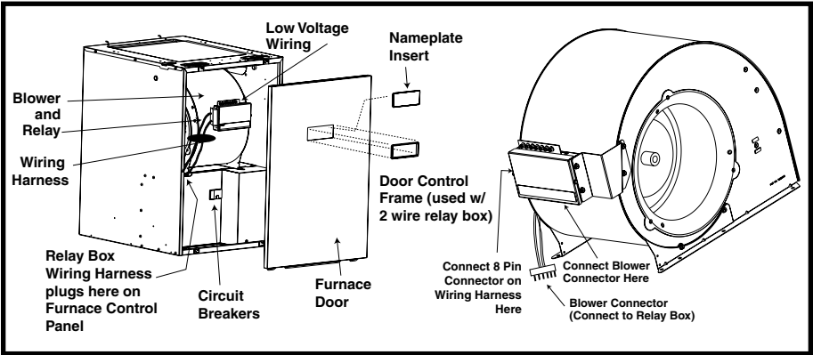
Figure 2a. E2E(-) Series Electric Furnace, manufactured prior to 1999
