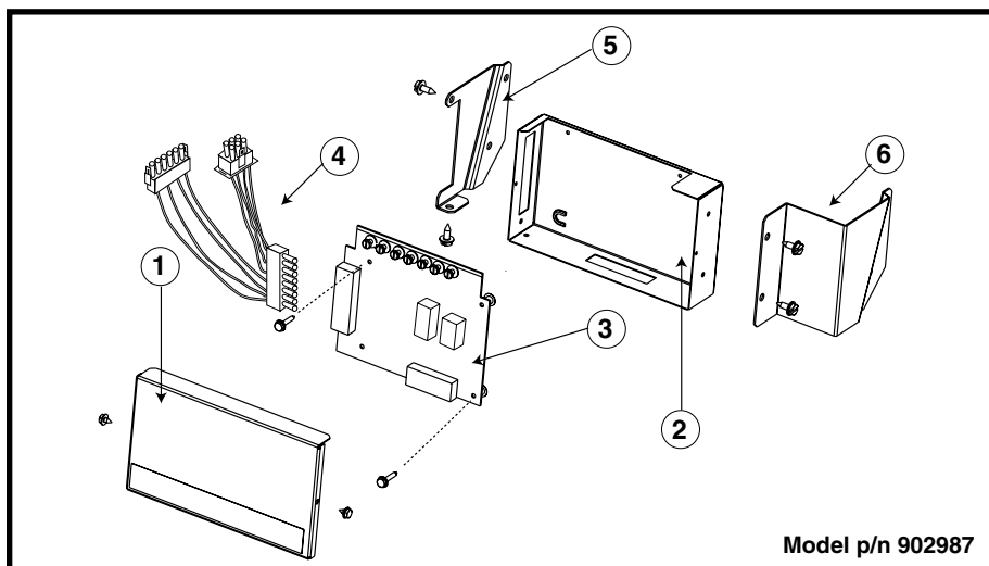
Figure 3. A/C Heat Pump Relay Box, Exploded View
