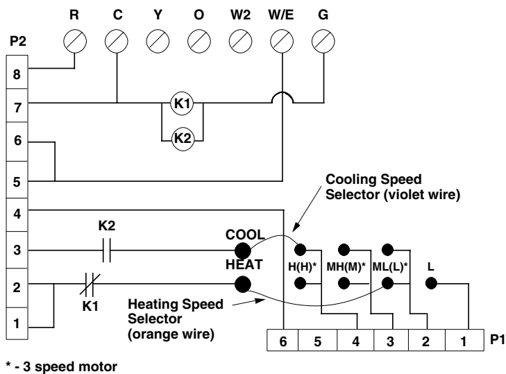
Figure 6. Wiring Schematics
