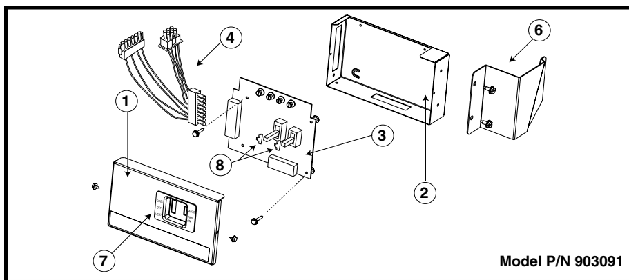
Figure 3. 2 Wire Relay Box, Exploded View
