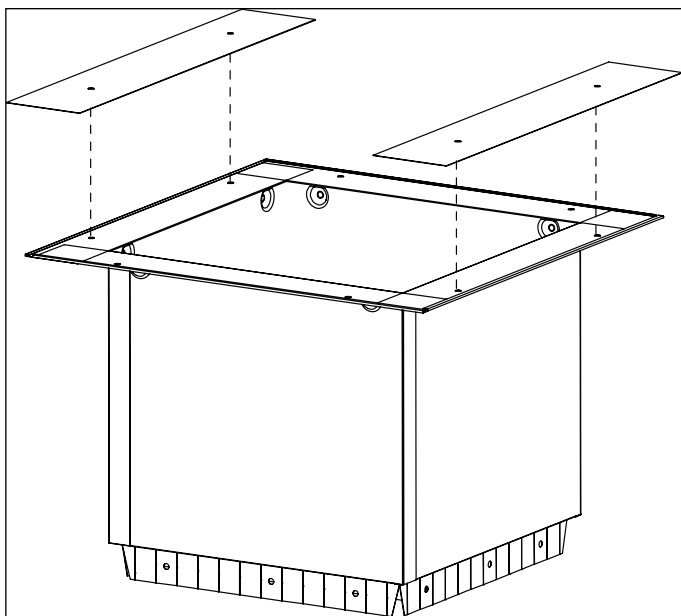
Figure 1. Duct Connector Preparation
