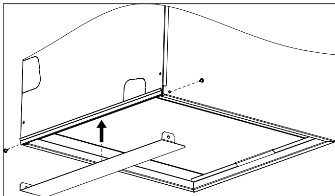
Figure 2. Coil Box Preparation
