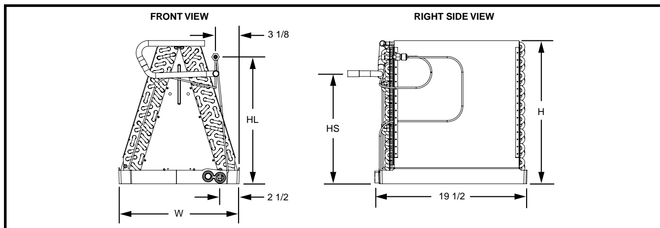
Figure 1. Coil Dimensions
