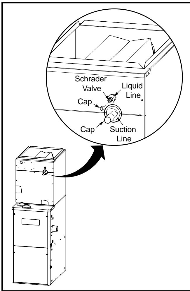
Figure 2. Suction & Liquid Line Locations
