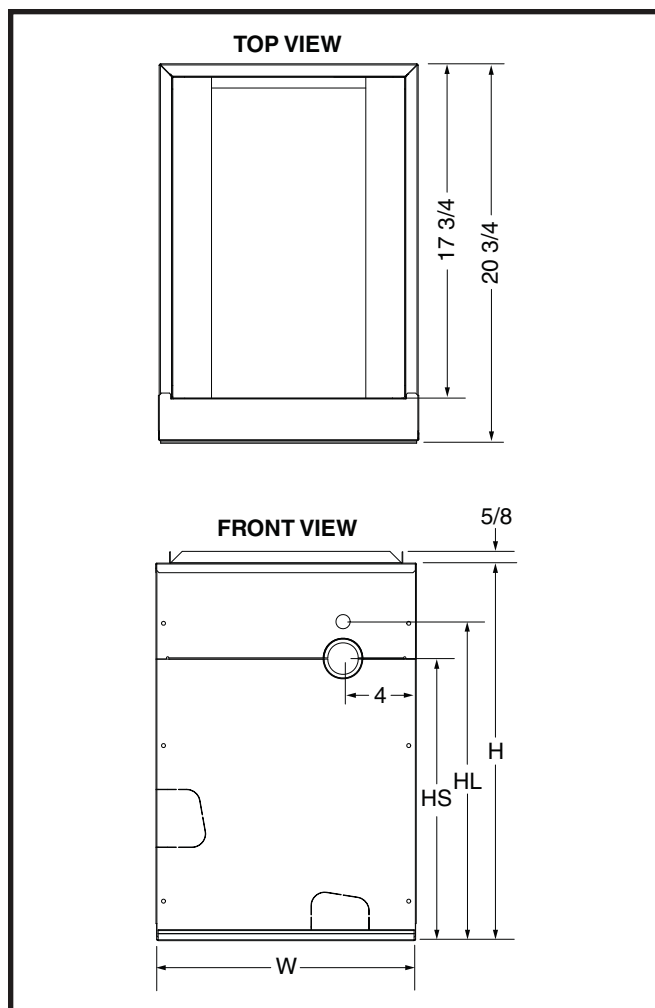
Figure 1. Coil Dimensions
