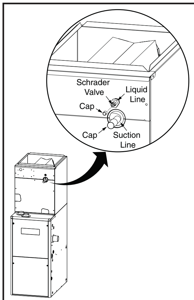
Figure 2. Suction and Liquid Line Locations
