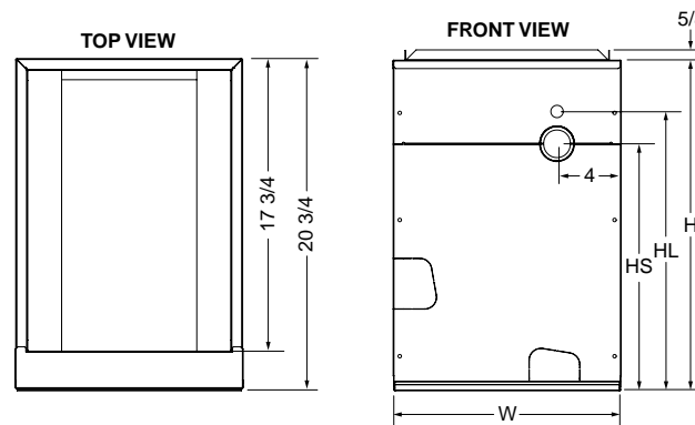
Figure 5. Coil Dimensions
