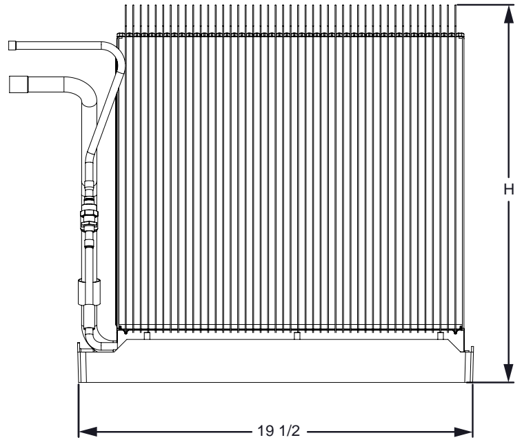
Figure 5. C7 Coil Dimensions
