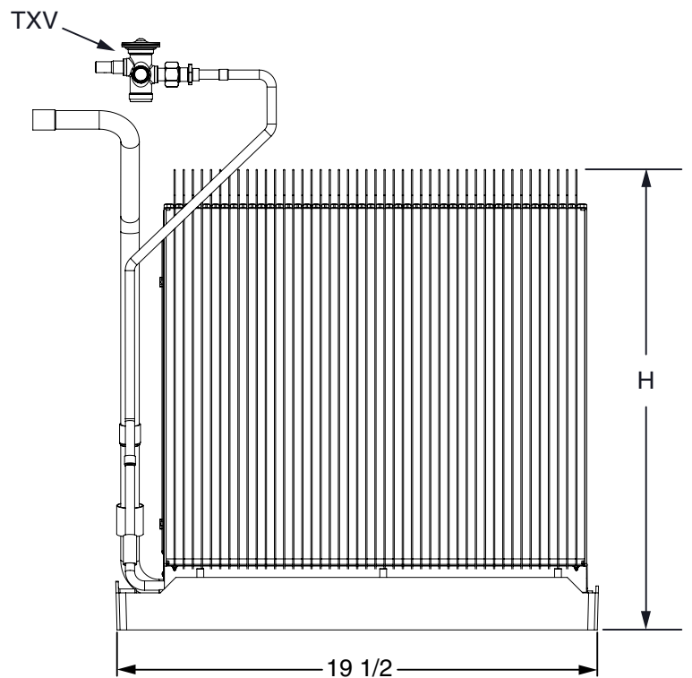
Figure 6. C7 Coil Dimensions (with TXV)
