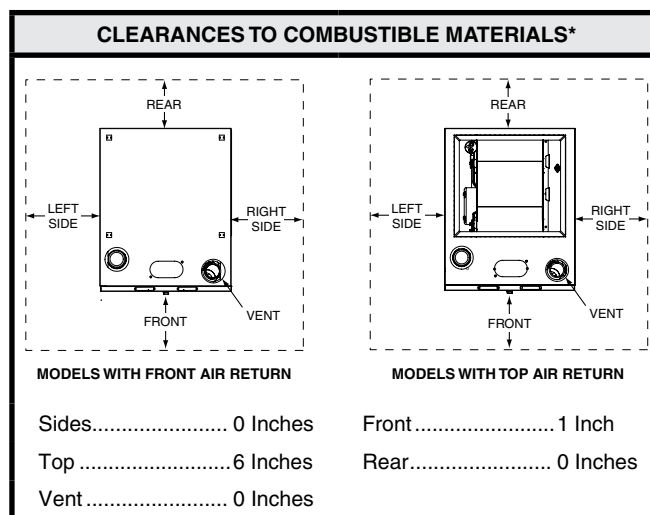
Figure 1. Minimum Clearances
