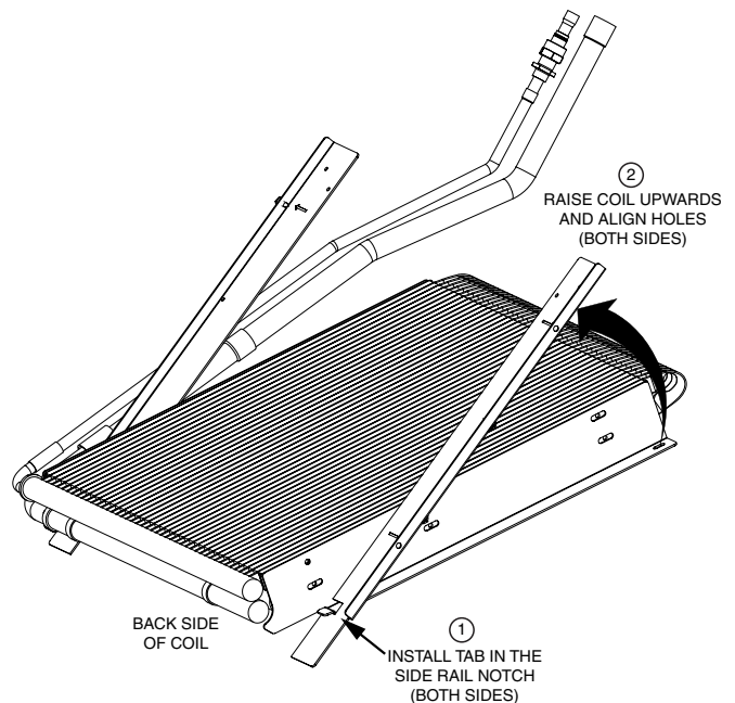
Figure 2. Coil Installation
