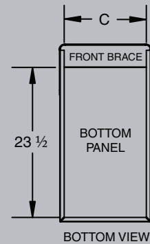
BOTTOM VIEW
